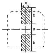
▨ Solder land on PC board
