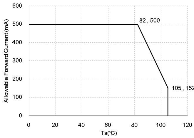
Allowable Forward Current vs. Case Temperature ( T_j < 115^\circ\text{C} )
