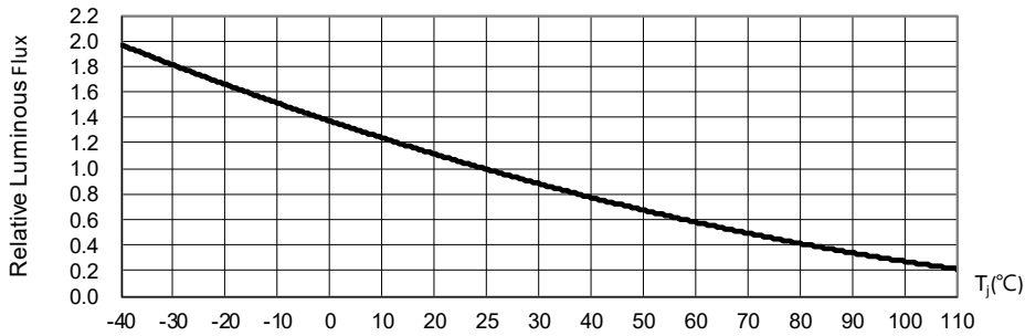
Fig. 5 Luminous Flux at I_F=50\text{mA} vs. Junction Temperature
