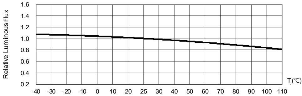
Fig. 5 Luminous Flux at I_F=140mA vs. Junction Temperature
