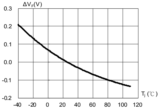
Fig. 3 Relative Forward Voltage vs. Junction Temperature \Delta V_F = V_F - V_F(25^\circ C) = f(T_s) ; I_F = 140mA
