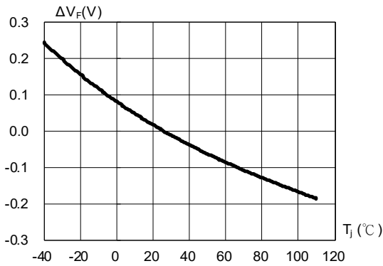
Fig. 3 Relative Forward Voltage vs. Junction Temperature \Delta V_F = V_F - V_F(25^\circ\text{C}) = f(T_j) ; I_F = 140\text{mA}
