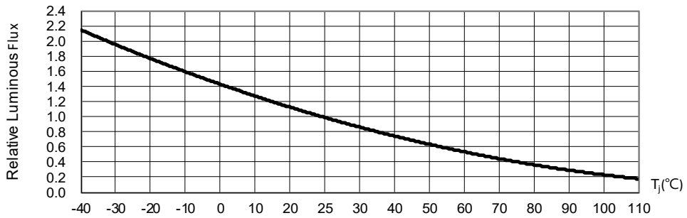
Fig. 5 Luminous Flux at I_F=140\text{mA} vs. Junction Temperature
