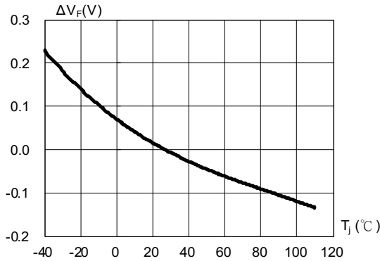
Fig. 3 Relative Forward Voltage vs. Junction Temperature \Delta V_F = V_F - V_F(25^\circ C) = f(T_s) ; I F = 140mA
