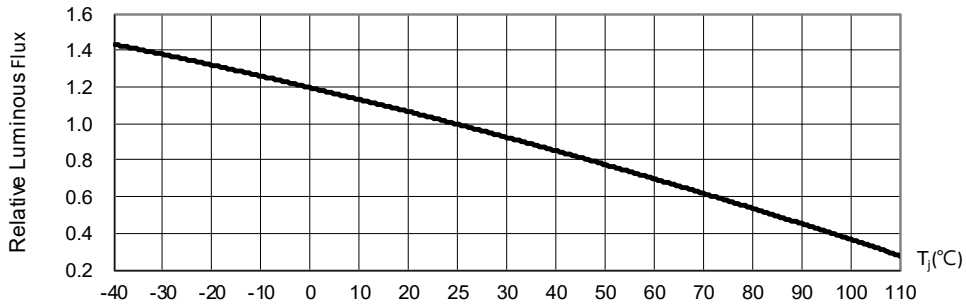
Fig. 5 Luminous Flux at I=140mA vs. Junction Temperature
