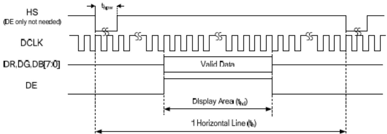
Fig1. Horizontal input timing at DE only mode
