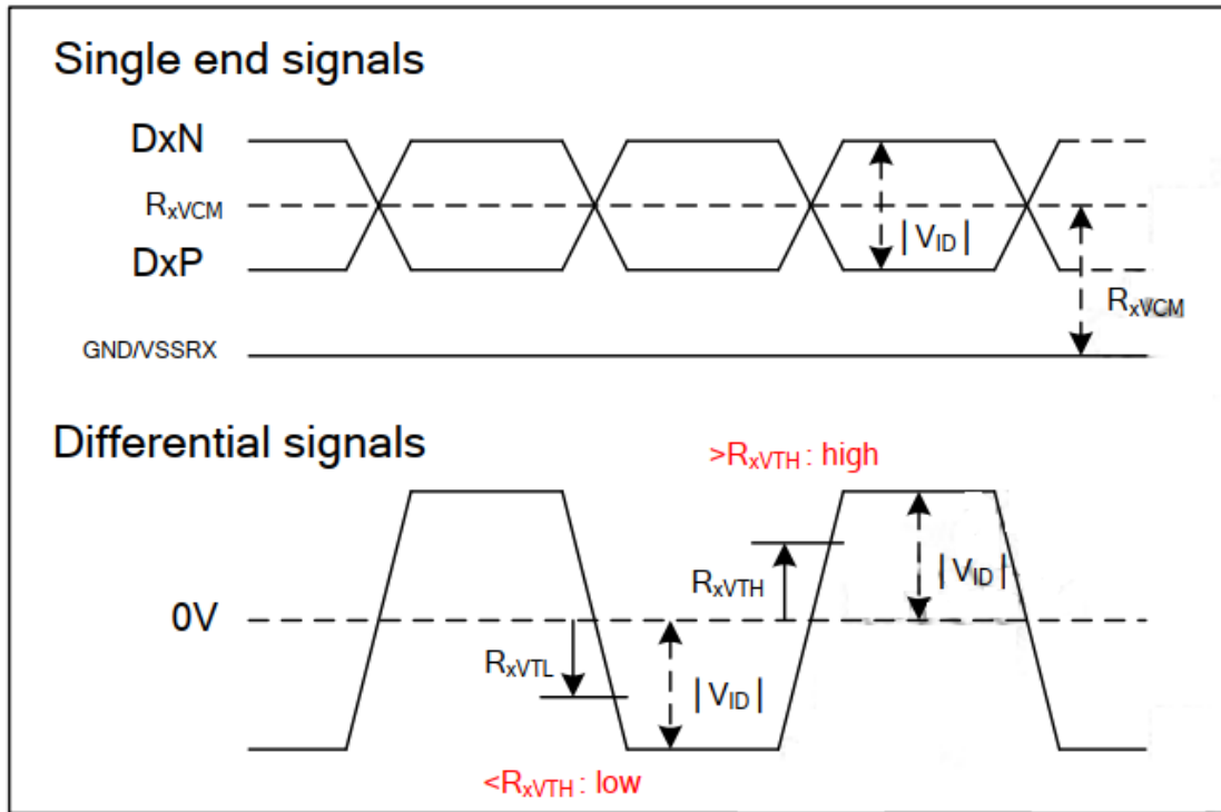
<Table 4. LVDS DC Timing Specification>
