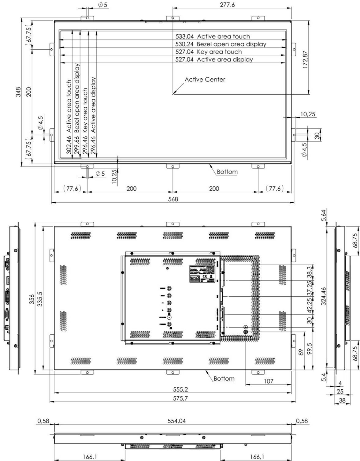
Figure 1: Mechanical Outlines
