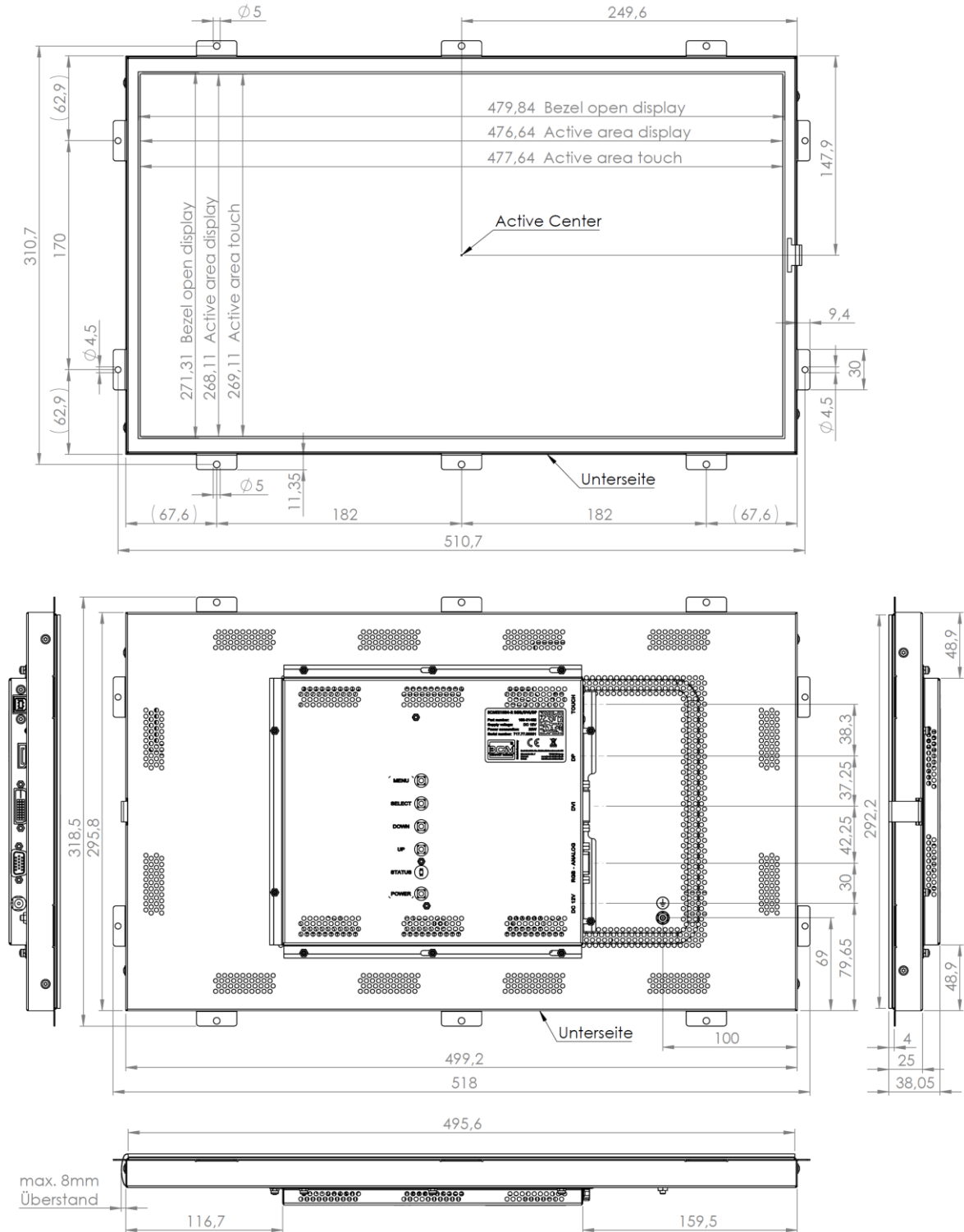
Figure 1: Mechanical Outlines
