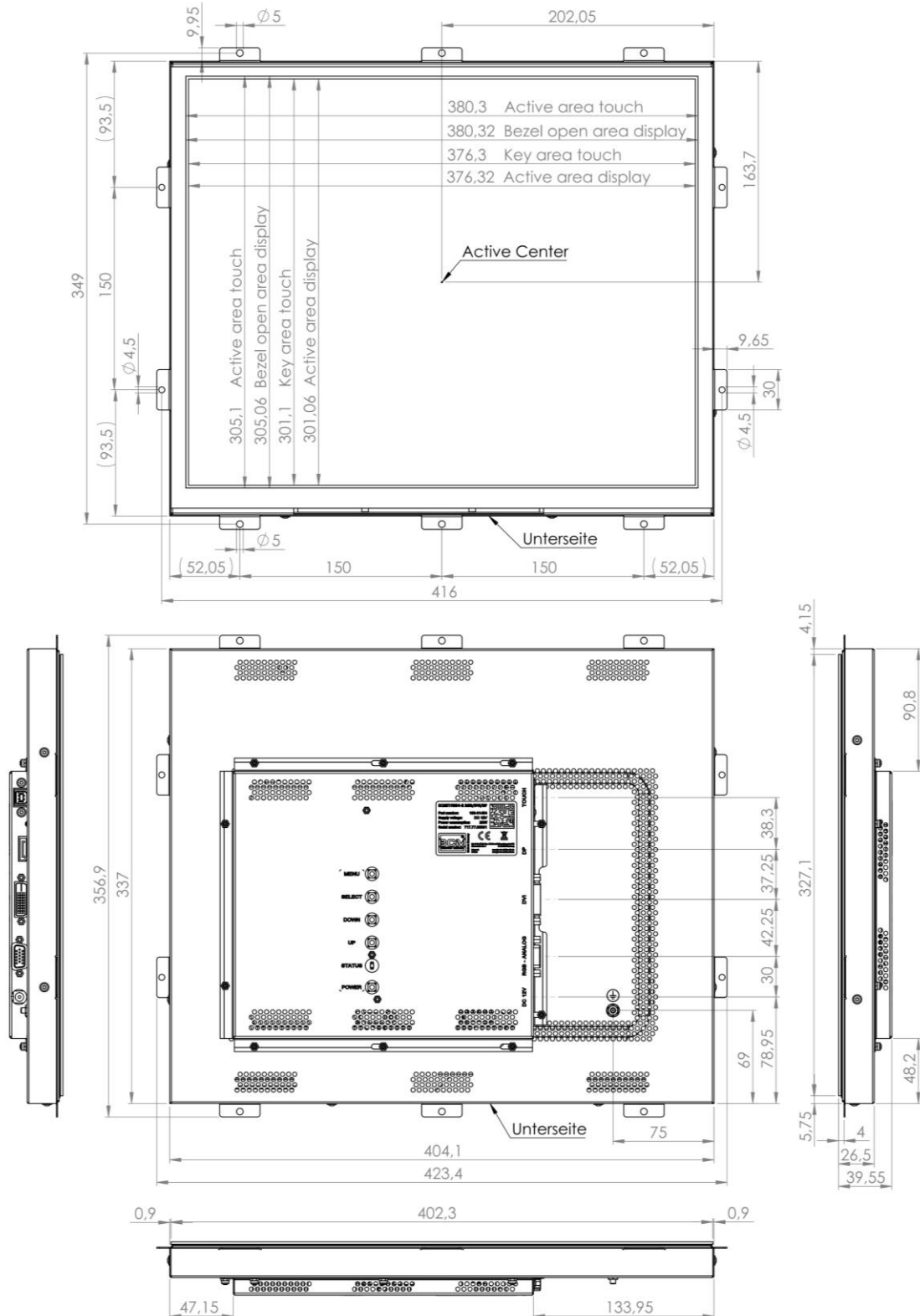
Figure 1: Mechanical Outlines
