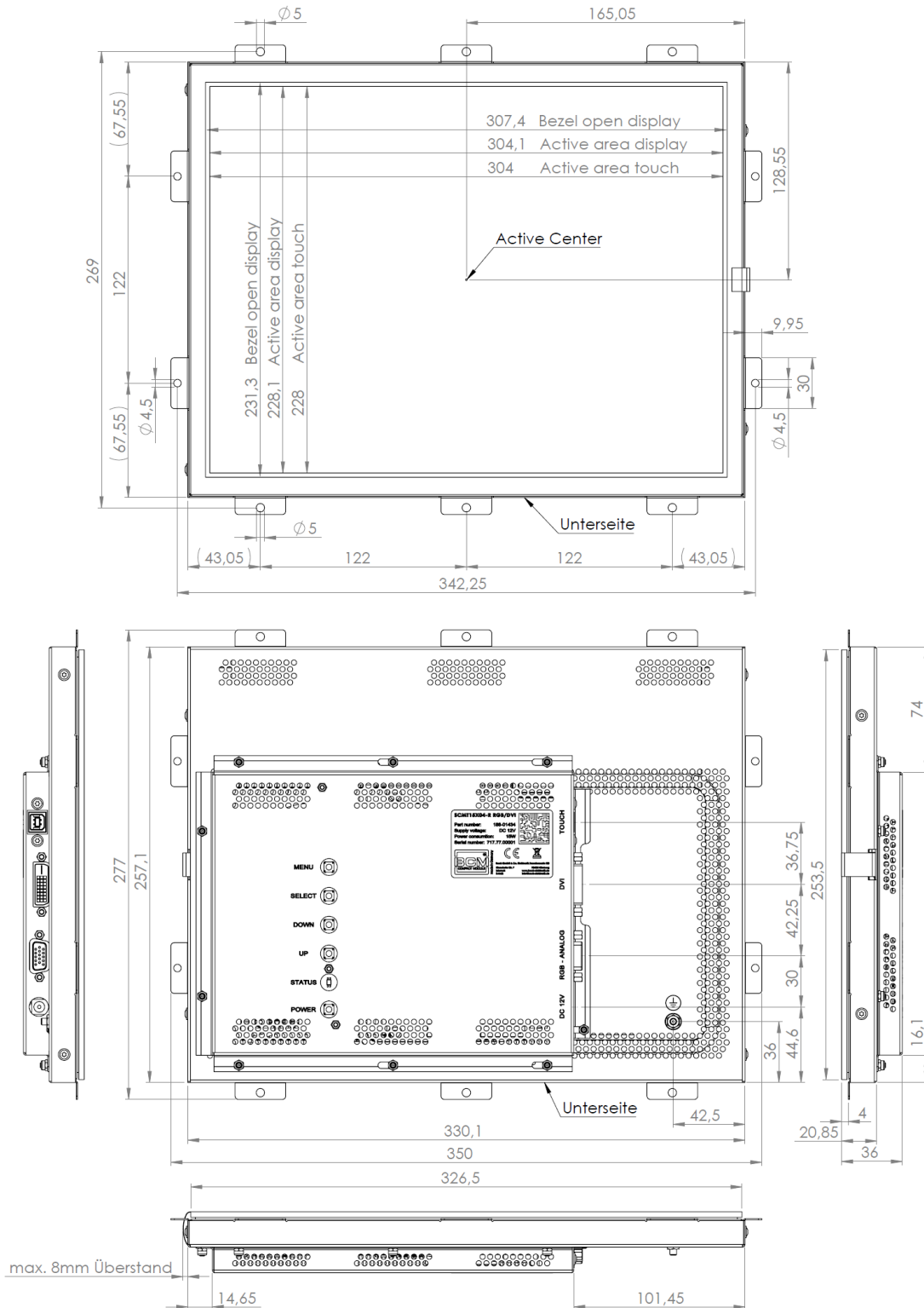
Figure 1: Mechanical Outlines
