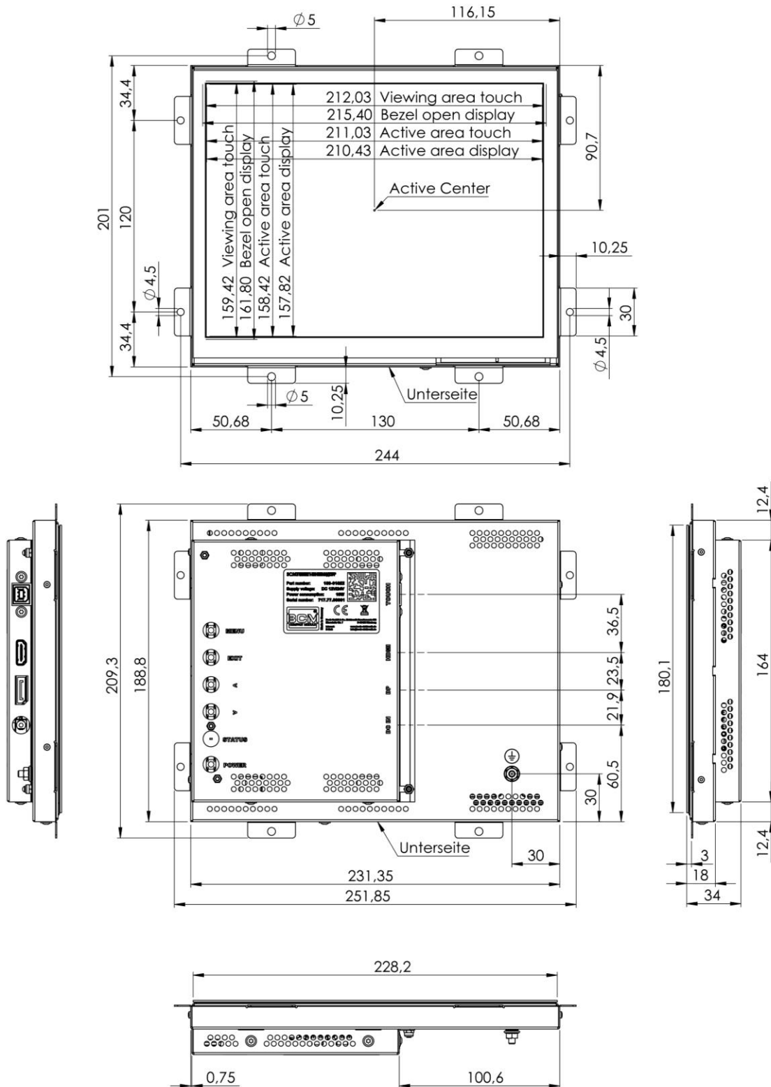
Figure 1: Mechanical Outlines
