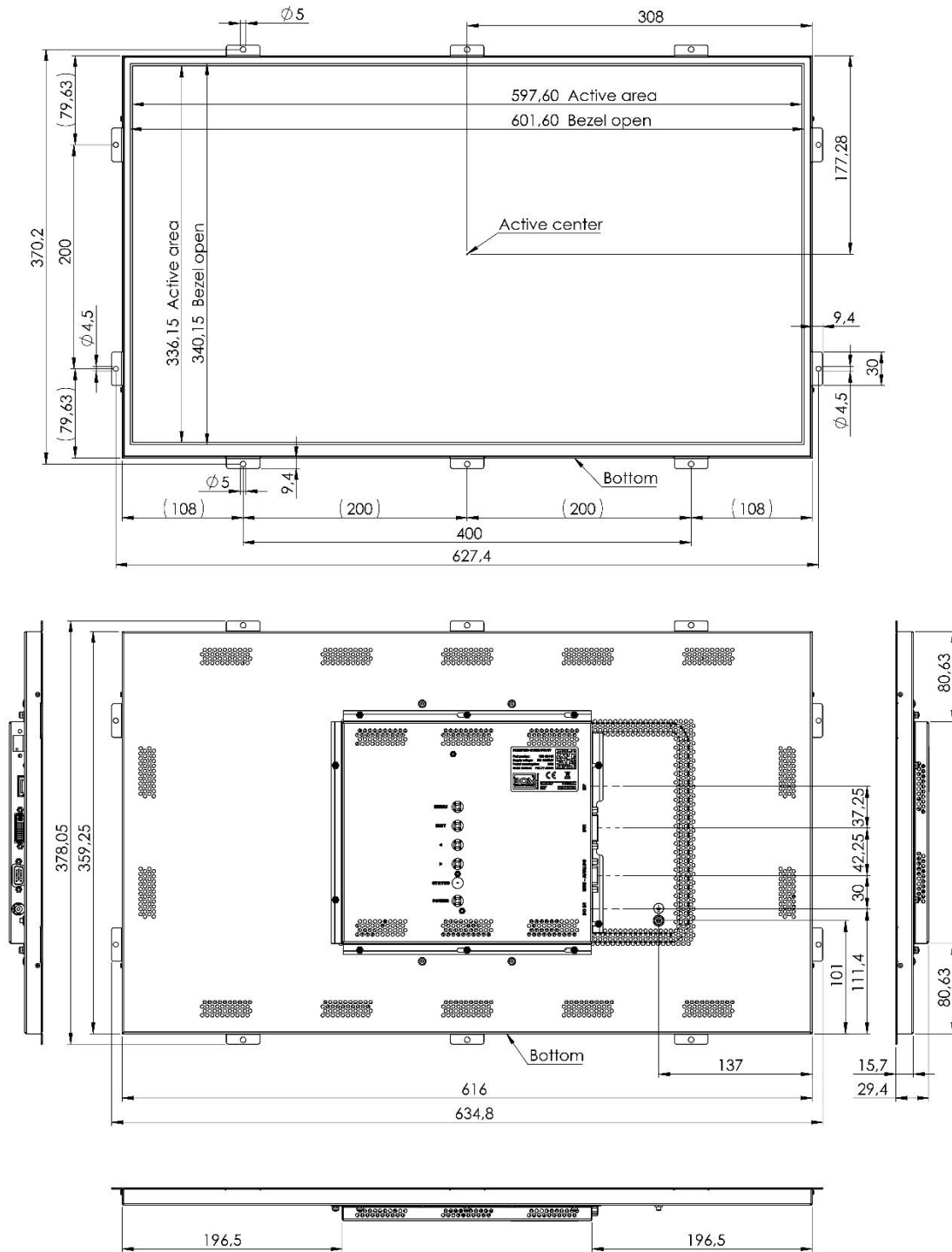
Figure 1: Mechanical Outlines
