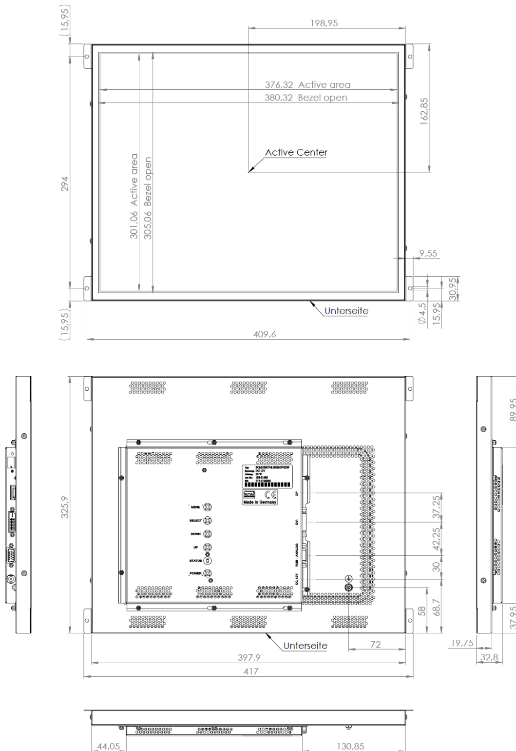
Figure 1: Mechanical Outlines
