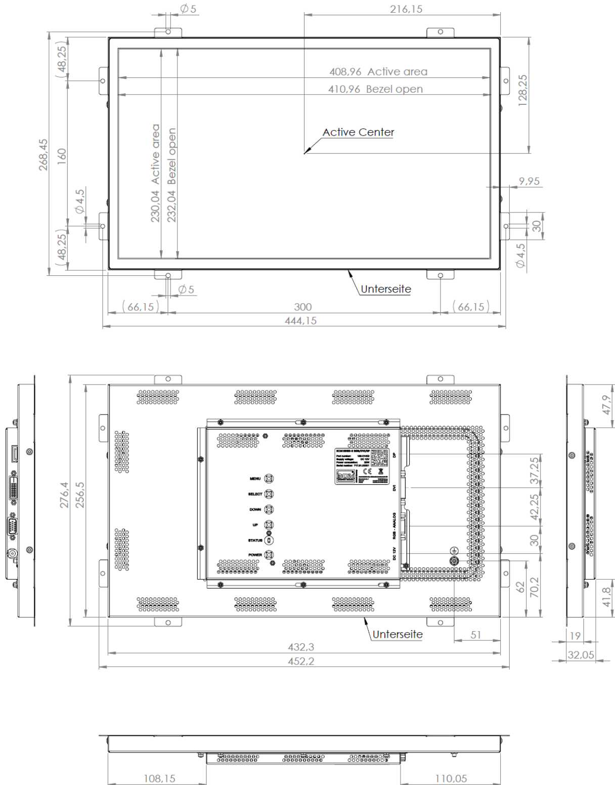
Figure 1: Mechanical Outlines
