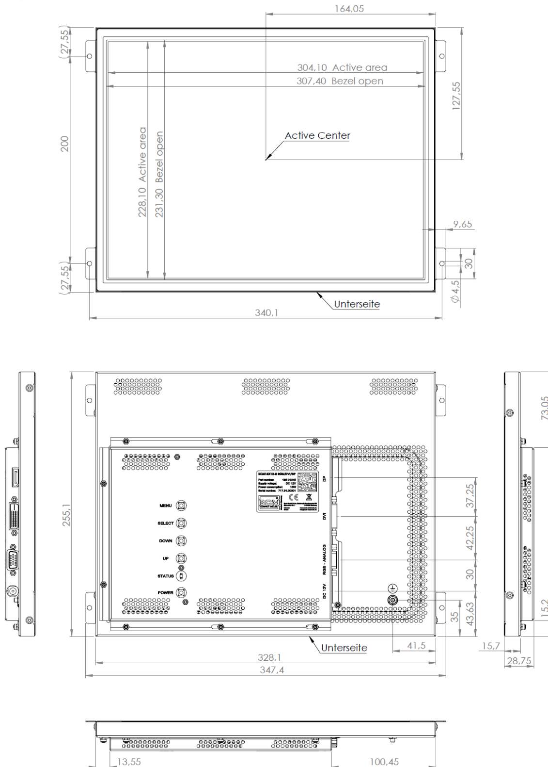
Figure 1: Mechanical Outlines
