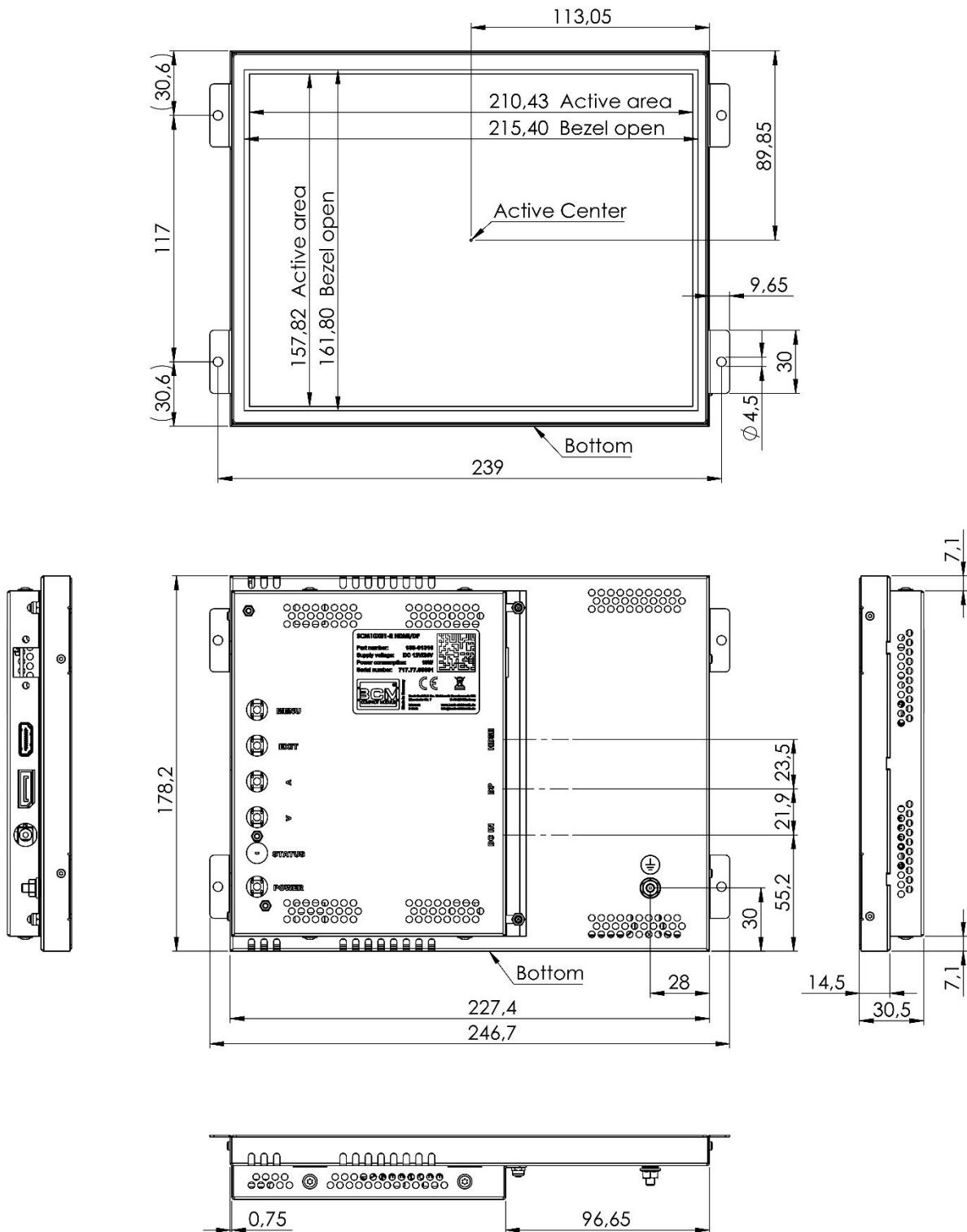
Figure 1: Mechanical Outlines
