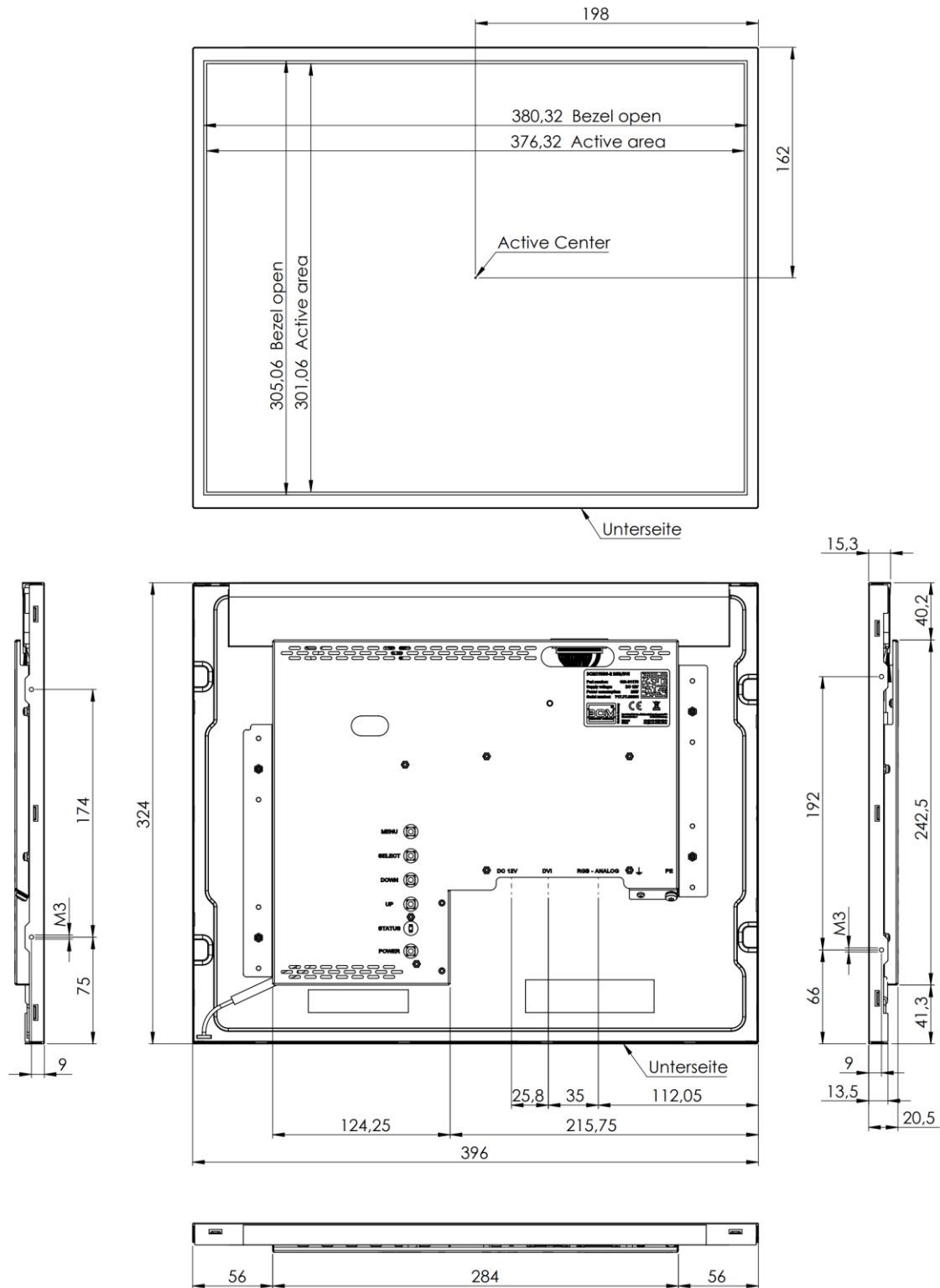
Figure 1: Mechanical Outlines
