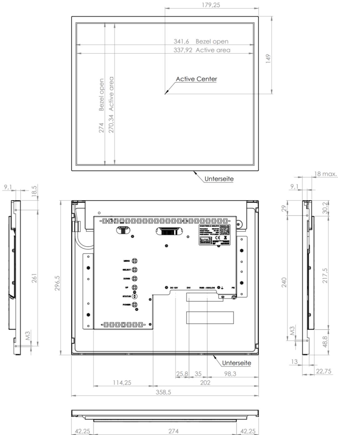
Figure 1: Mechanical Outlines
