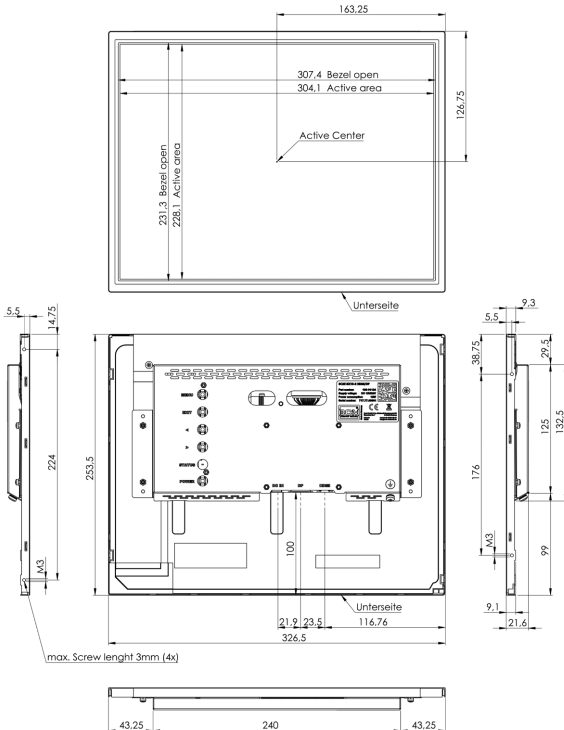
Figure 1: Mechanical Outlines
