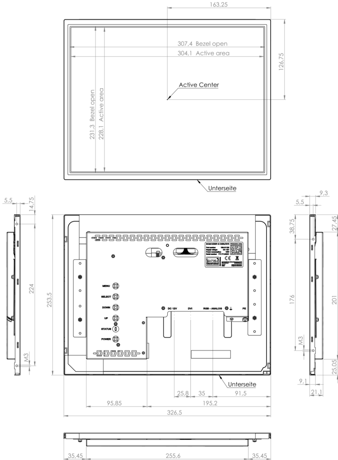
Figure 1: Mechanical Outlines
