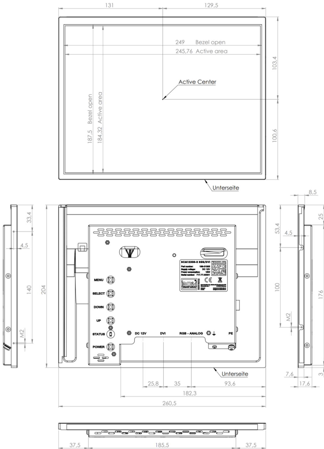
Figure 1: Mechanical Outlines
